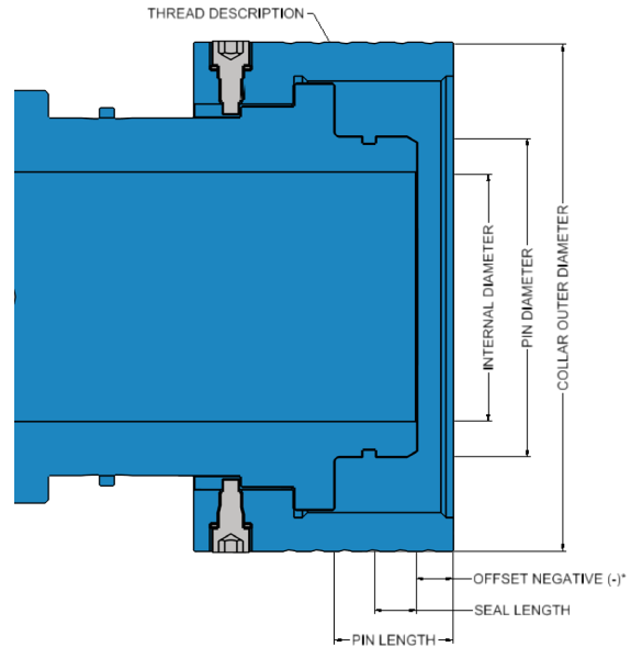
QUICK UNION REQUIRED INFORMATION *OFFSET FROM COLLAR TO END OF PIN IS SHOWN HERE AS A NEGATIVE SIZE
