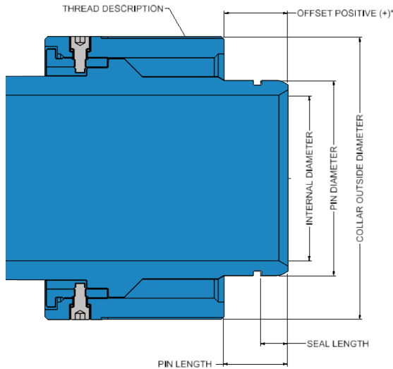
QTS PIN REQUIRED INFORMATION *OFFSET FROM COLLAR TO END OF PIN IS SHOWN HERE AS A POSITIVE SIZE
